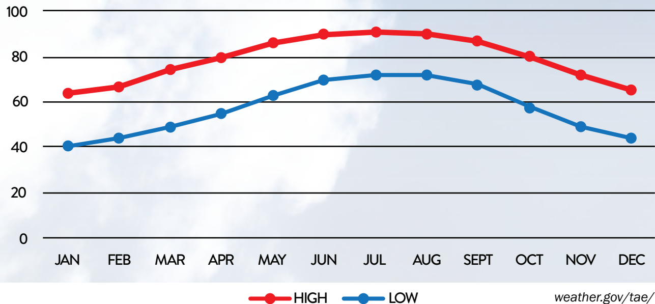
TLH AVERAGE DAILY LOWS AND HIGHS (IN FAHRENHEIT, 1991-2020)
